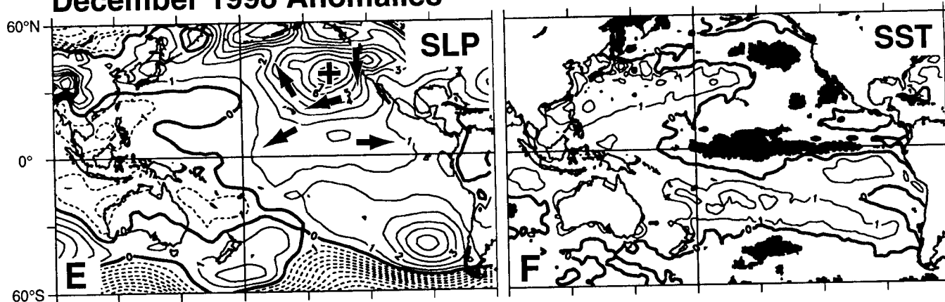
Figure 4. Anomalies over the Pacific Ocean for May, September, and December of 1998: A, C, and E, sea-level pressure (SLP) with anomalous surface wind; B, D, and F, sea-surface temperature (SST). Positive anomalies denote higher than normal atmospheric pressure and warmer than normal SST. Contour intervals are 1 mb and 1°C. Shading denotes SST anomalies greater than 1°C. Arrows indicate the direction and strength of the wind anomalies. Anomalous surface winds are approximately parallel with SLP contours, and cyclonic (counterclockwise in Northern Hemisphere) around negative anomalies. Closer-spaced SLP contours indicate faster anomalous winds. Monthly data were obtained from the Climate Diagnostics Center. The SLP climatology period is 1968–96; the Reynolds SST climatology period is 1950–79.
