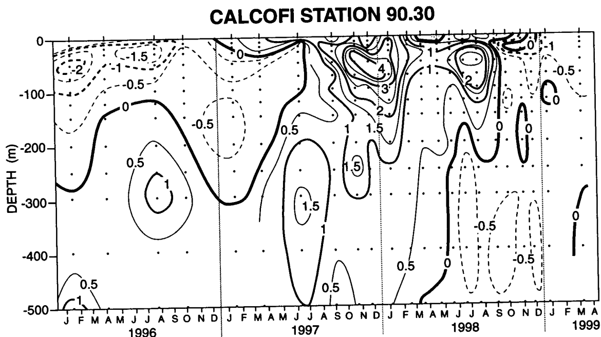
Figure 17. Anomalies in temperature ( ^{\circ}\text{C} from the 1950–92 base period) versus depth and time for CalCOFI station 90.30.
