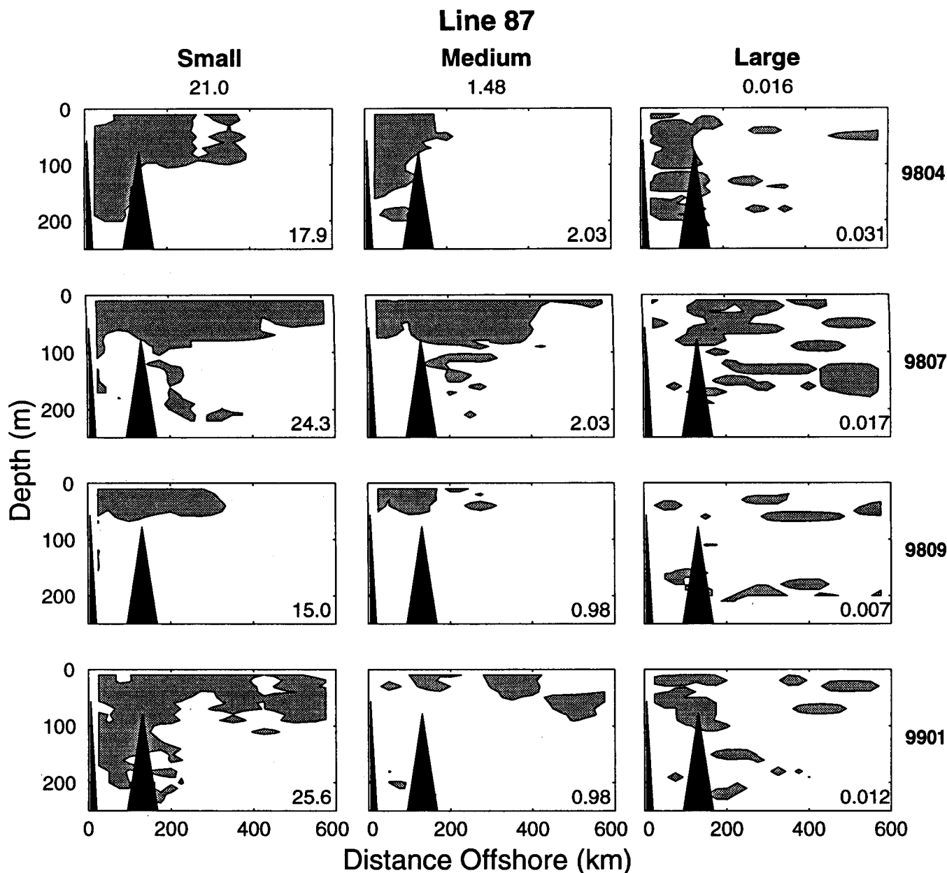
Figure 32. Optical plankton counter (OPC) data for line 87. Shown is particle concentration (particles liter -1 ) for small (0.266–0.722 mm ESD, left panels), medium (0.722–2.38 mm ESD, center panels), and large (2.38–14.0 mm ESD, right panels) particles for four cruises (indicated at right). For each panel, particle concentration is shown in relation to distance offshore and depth. The number at the top of each column of panels is the mean particle concentration for all four cruises for the respective particle size class. The number in the lower right corner of each panel is the mean particle concentration within each cruise for the respective size class. The shaded regions in the panels represent particle concentrations greater than the mean concentration for all cruises for the respective size class.
