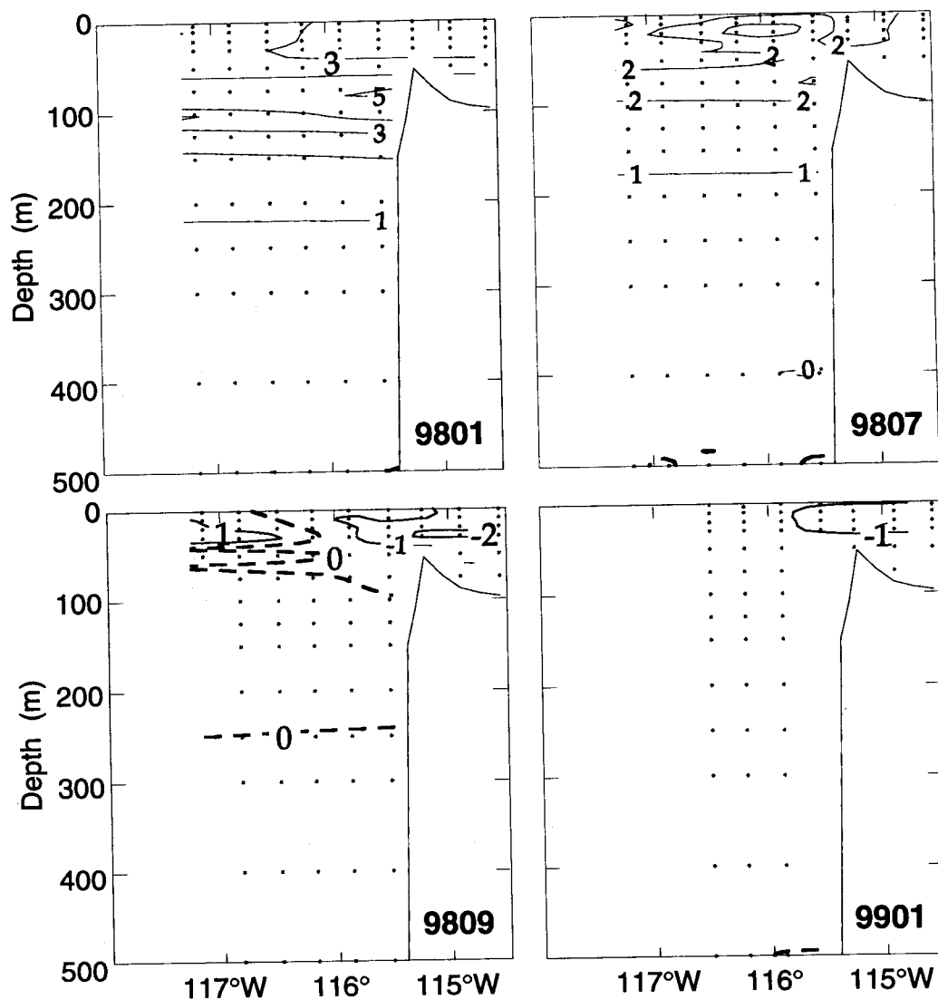
Figure 24. Temperature anomalies ( ^{\circ}\text{C} ) for line 120 from IMECOCAL cruises 9801, 9807, 9809, and 9901. Anomalies were calculated from mean values given by Lynn et al. (1982) for the period 1950–78.
